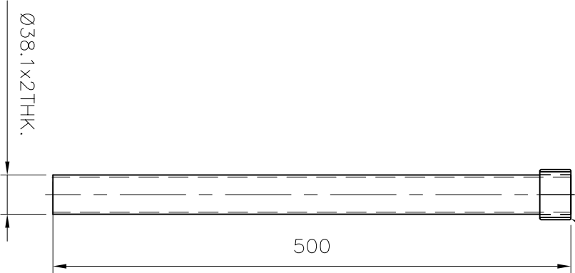
DETAIL OF STRAIGHT PIPE
