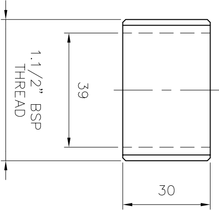
(SCALE-1:4) DETAIL-A BUSH FOR COUPLER
